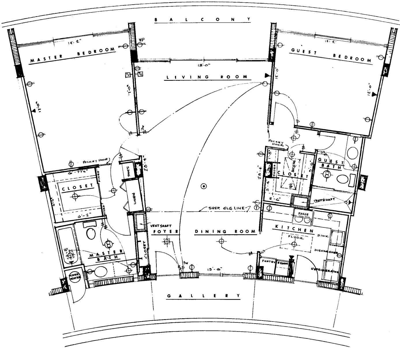
TYPICAL APARTMENT TYPE A 03,05,07,09.
